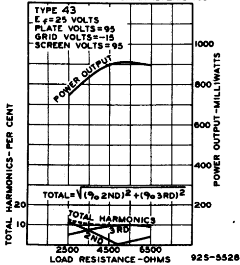
AVERAGE OUTPUT CHARACTERISTICS
